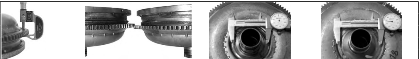
HO77 - .355" Thick Ring Gear HO78 - .275" Thick Ring Gear HO77 - 2.600" Flanged Impeller Hub HO78 - 3.075" Flanged Impeller Hub
